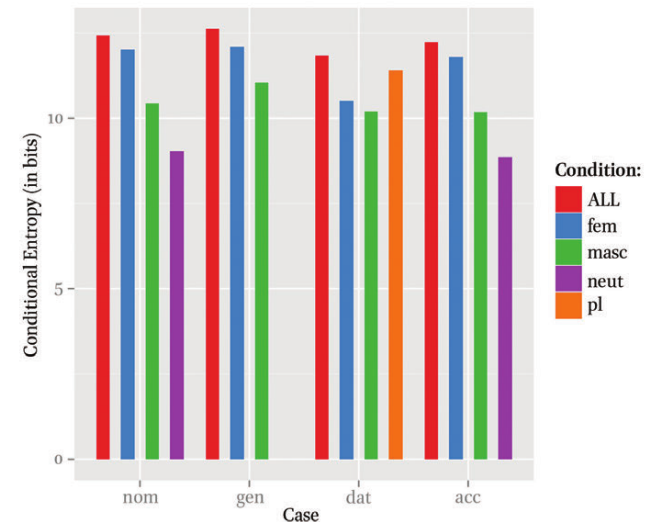
Figure. Noun entropy conditioned on case and number.
