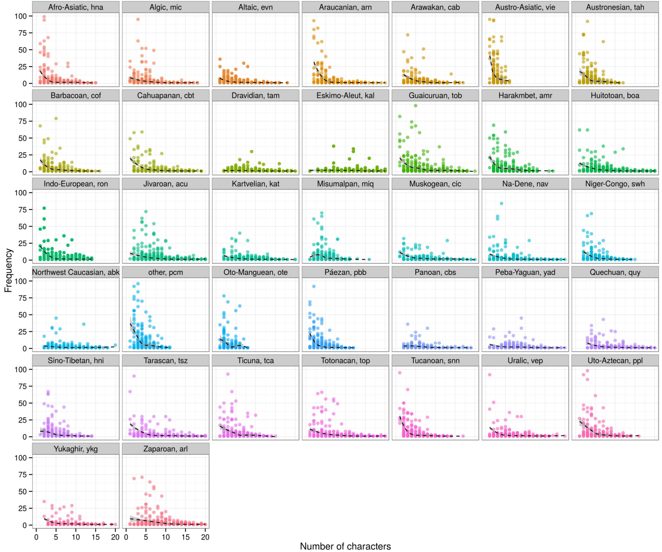
Fig. 1. The relationship between frequency of occurrence (y-axis) and number of characters (x-axis) for different language families in the UDHR. The languages selected represent the mode of kendall's \tau values across all the languages of the family. For illustration purposes, a LOESS smoother with 95% confidence intervals is added (dashed black). The grey boxes above plots give names of language families and the ISO 639-3 codes for languages chosen to represent them.
